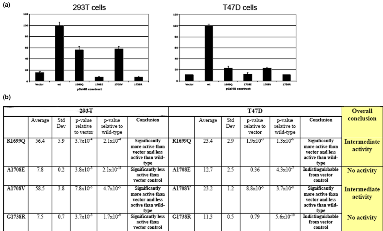
Transcriptional transactivation by C-terminal BRCA1 variants. (a) Graphical representation of results. Values are the mean and standard deviation of triplicate transfections. (b) Table showing means, standard deviations, and p values relative to vector and wild-type (wt) controls.
